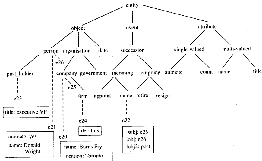
Figure 5: A Fragment of the LaSIE Discourse Model
