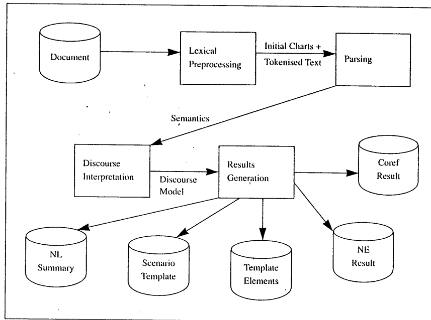
Figure 2: LaSIE System Architecture
